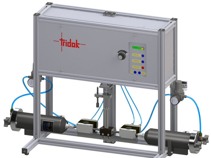
Model 1200 outfitted with two 20 oz Cartridge Retainers (Reservoirs are not included on standard system)
