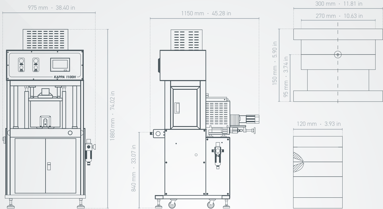
Machine
